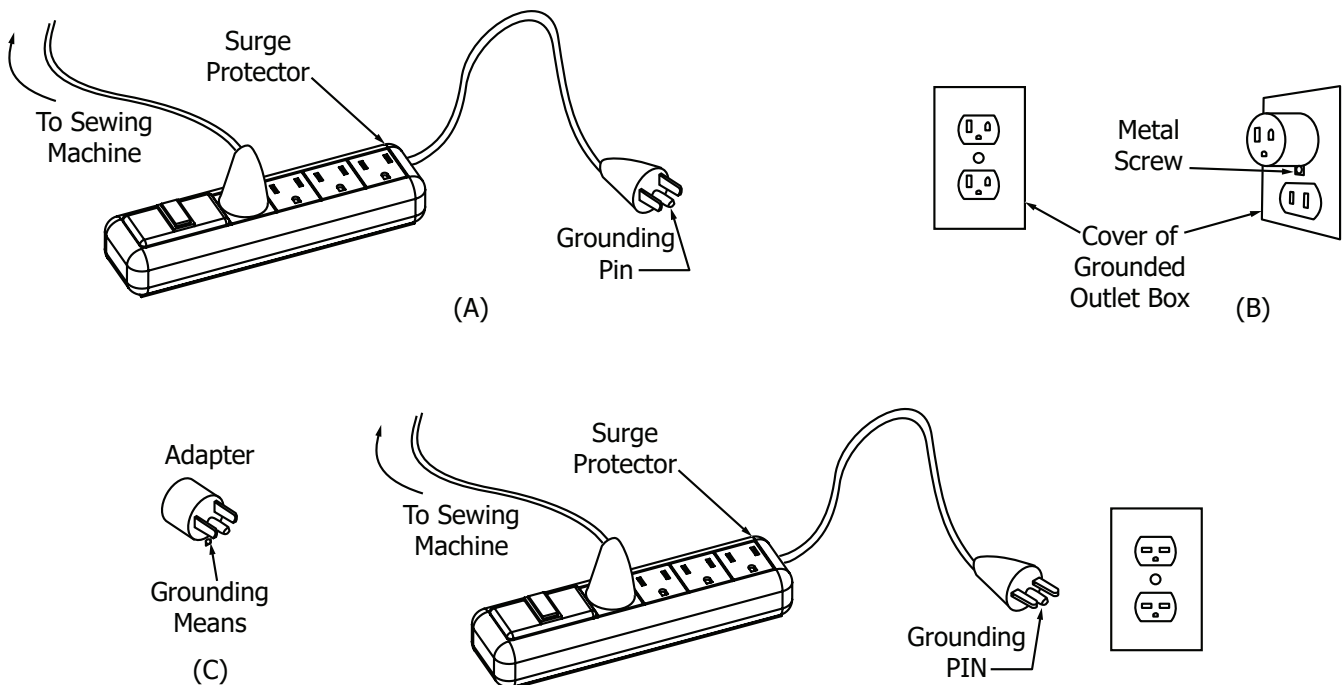
Grounding Methods
